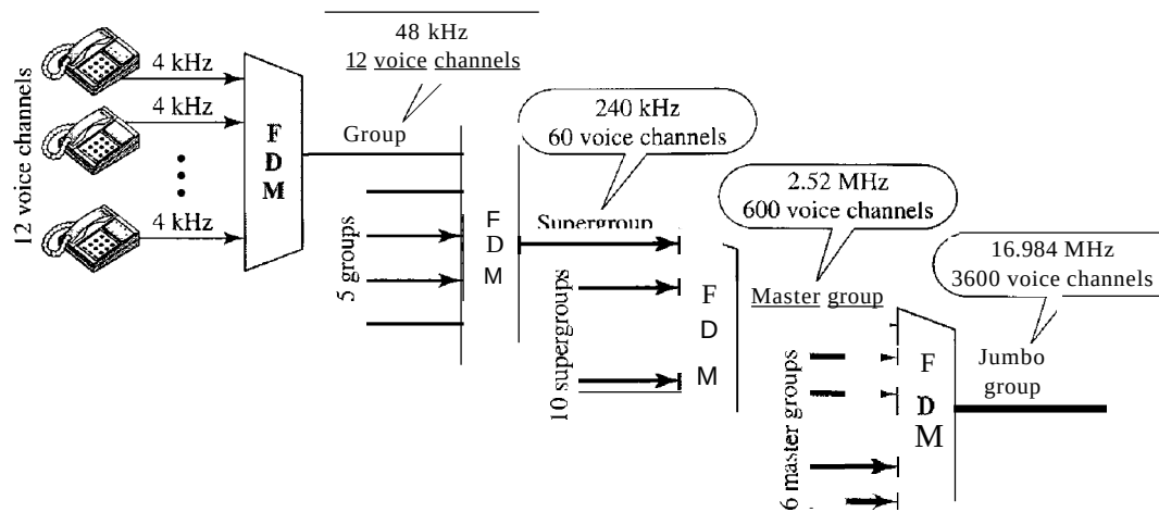
Figure 6.9 Analog hierarchy
