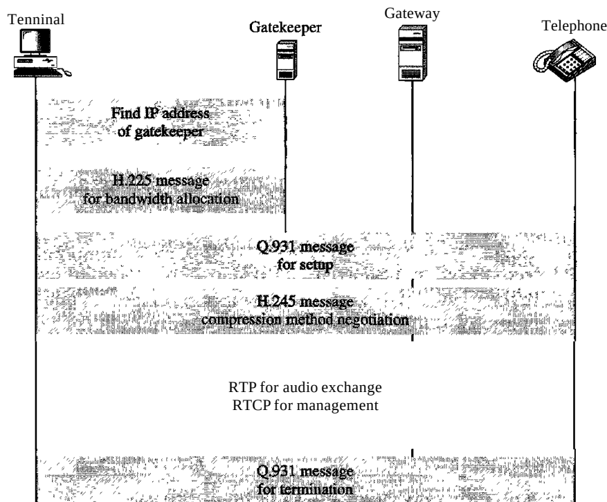
Figure 29.27 H.323 example
