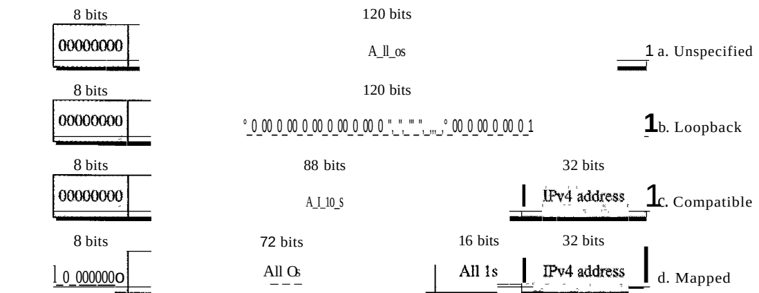
Figure 19.18 Reserved addresses in IPv6
