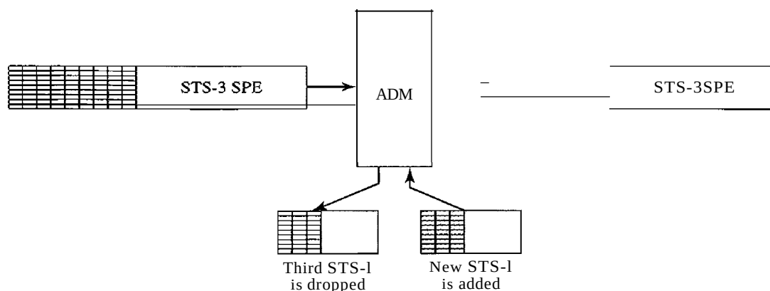
Figure 17.16 Dropping and adding STS-1 frames in an add/drop multiplexer
