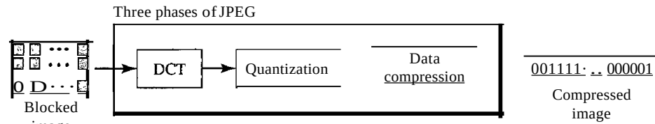
Figure 29.3 IPEG process
