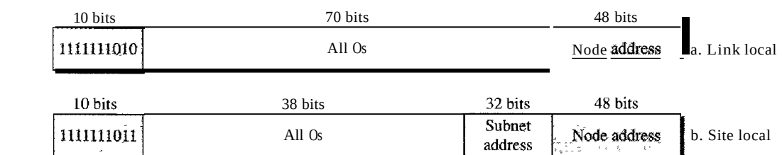
Figure 19.19 Local addresses in IPv6
