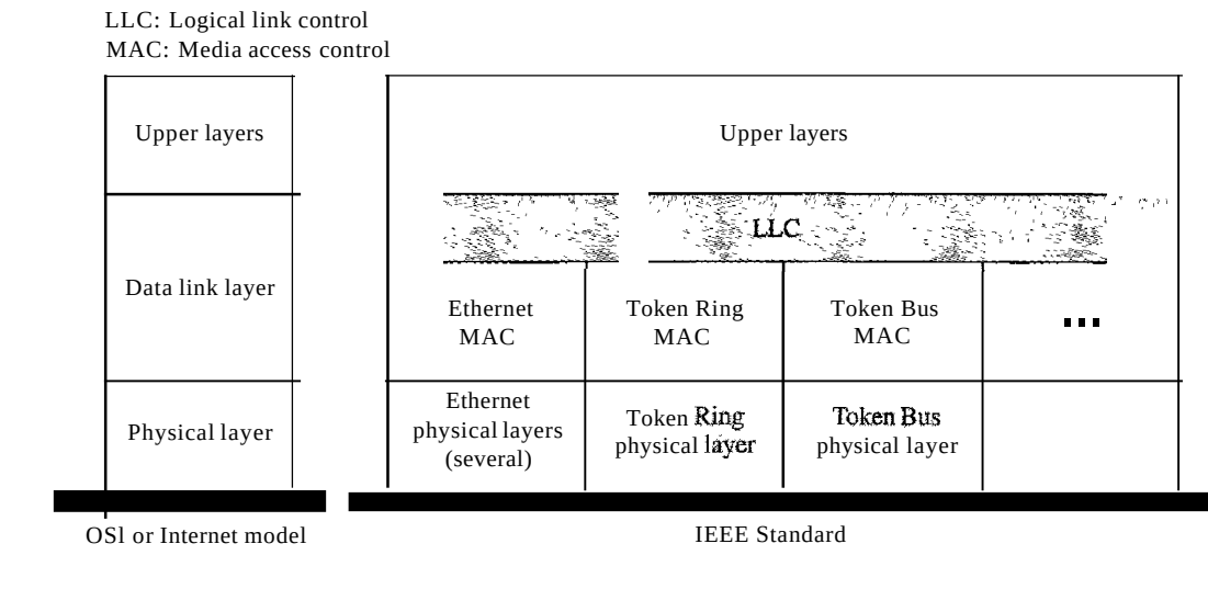
Figure 13.1 IEEE standard for LANs
